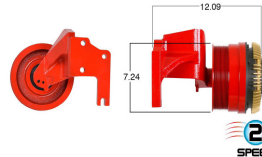
Part # 99782-2 Cummins ISX 15W
