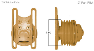
Part # 90007 Caterpillar 3406
