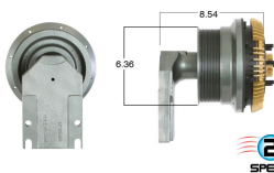
Part # 99590-2 PACCAR MX13WW
