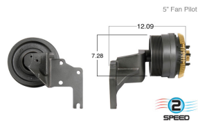
Part # 99589-2 Cummins ISX 15
