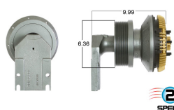
Part # 99592-2 PACCAR MX13
